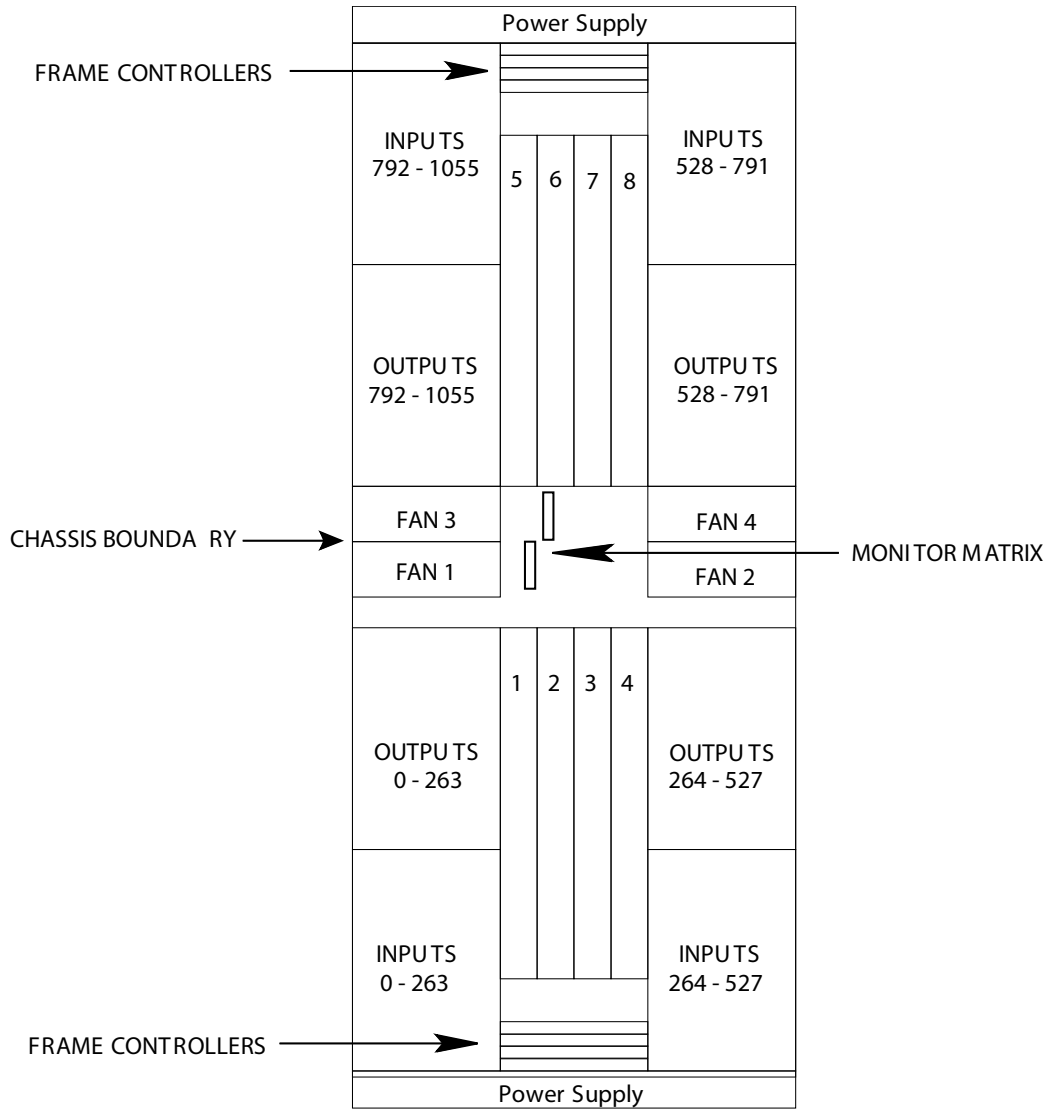
FIGURE 1-3. The Utah-400 XL Configuration
