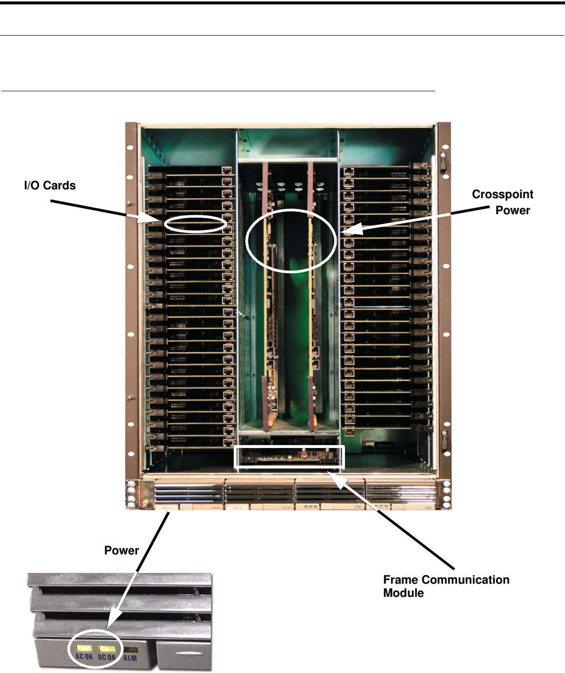
FIGURE 2-33. 288 Systems
