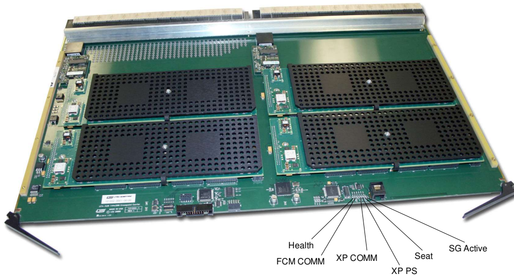
FIGURE 3-9. Crosspoints LEDs
