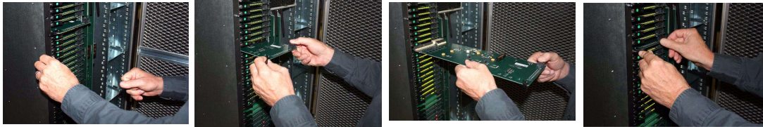
FIGURE 3-10. Input/Output Board Replacement and Removal
