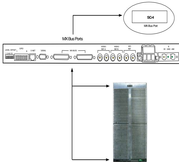
FIGURE 2-23. The MX-Bus Installation to an SC-4 Controller
