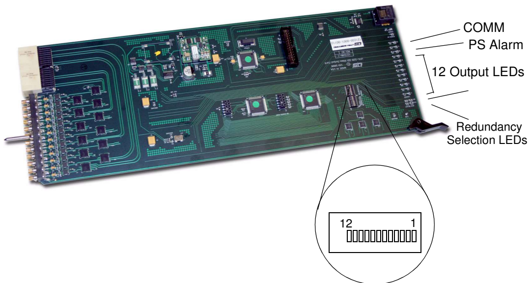
FIGURE 4-2. Multi-rate Output Board
