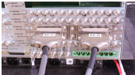
FIGURE C-4. Analog inputs
