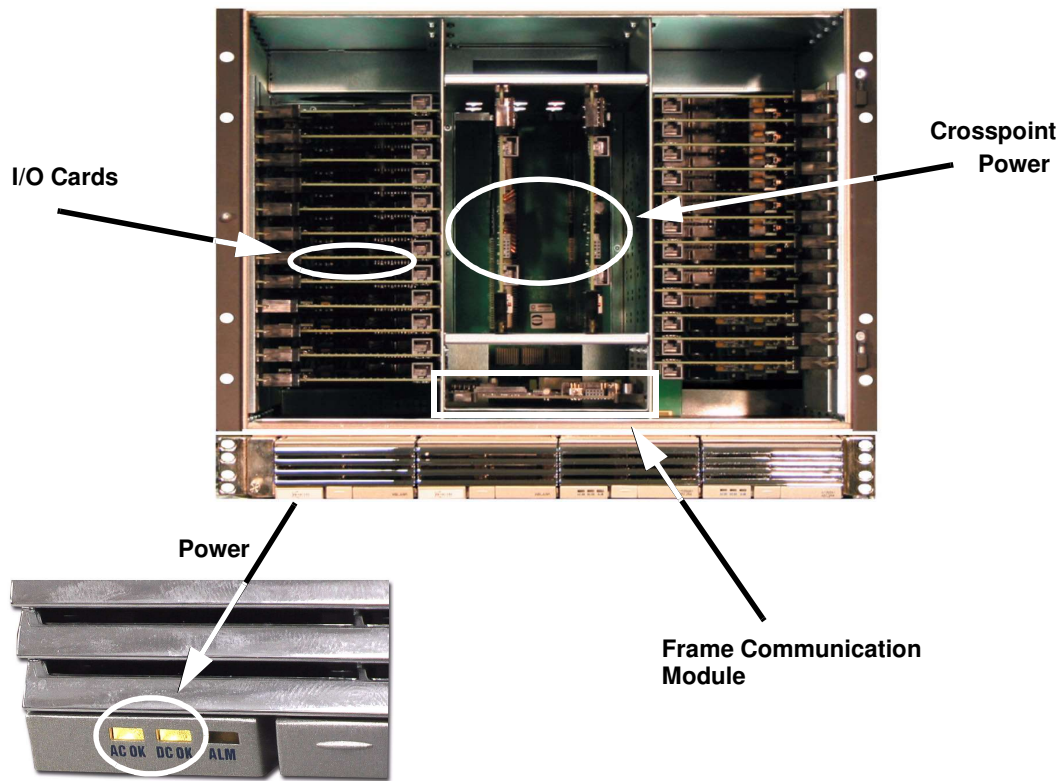
FIGURE 2-32. 144 Systems
