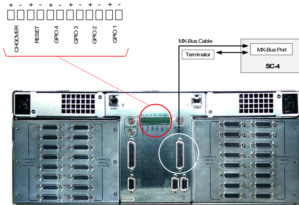
FIGURE 2-5. The MX-Bus Installation to an SC-4 Controller
