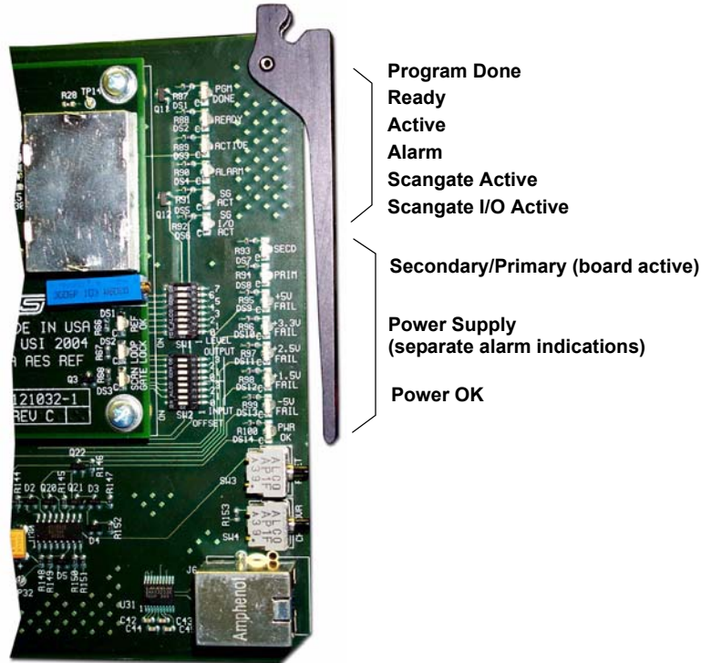
FIGURE 4-28. Crosspoint Board LEDs
