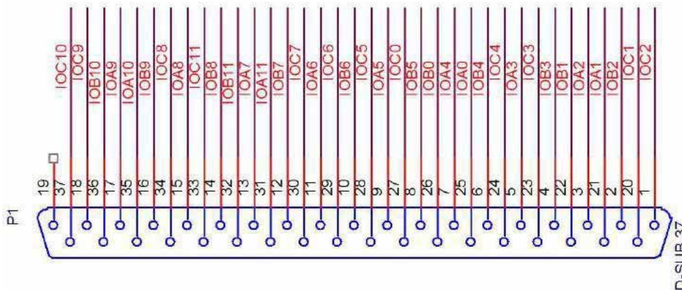
Rear Panel Pinout (2xD-Sub 37).
