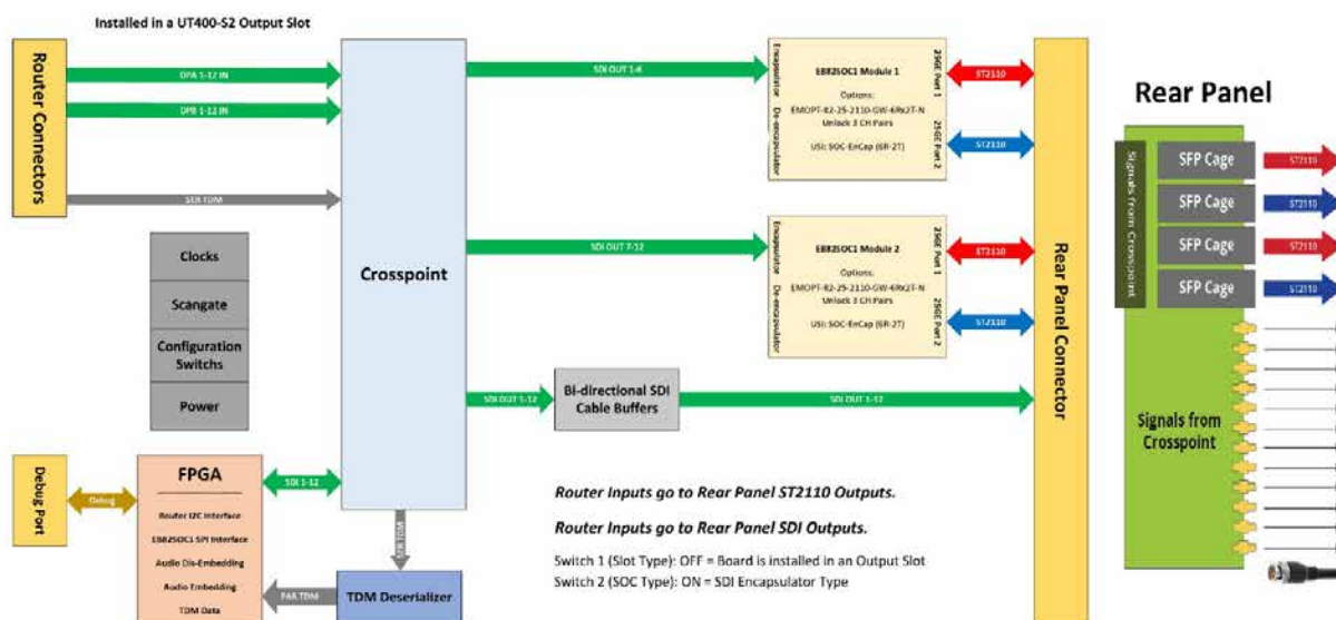
SDI-IP Passthrough Version 3 - PCB Block Diagram (SDI Output, ST2110 Output)
