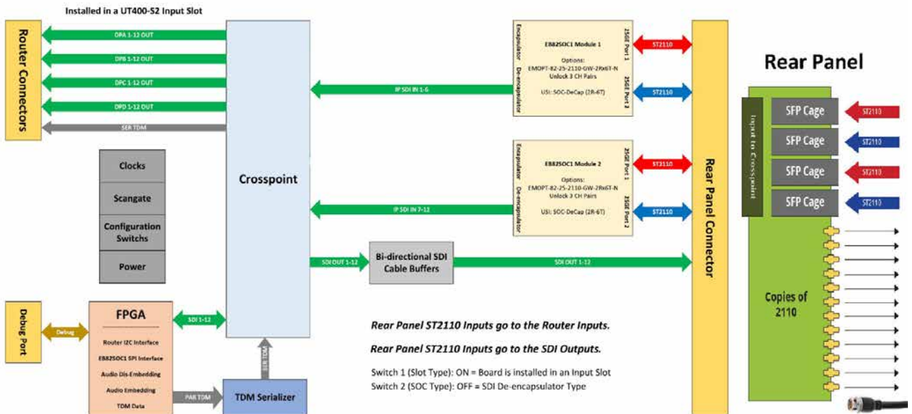
SDI-IP Passthrough Version 3 - PCB Block Diagram (ST2110 Input, SDI Output)
