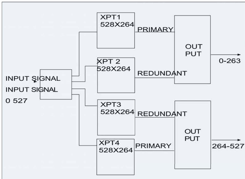
528 x 528 Matrix Block Diagram
